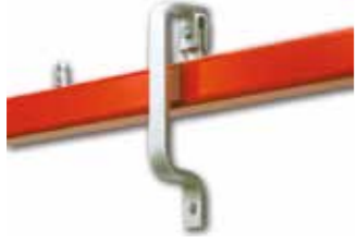
Ters Askılama Reverse Hanger
